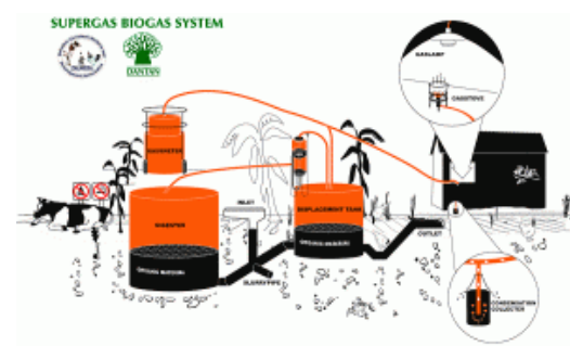
SUPERGAS BIOGAS SYSTEM
